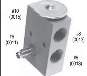
EXPANSION VALVE
